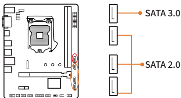
2-10 SATA Interface
