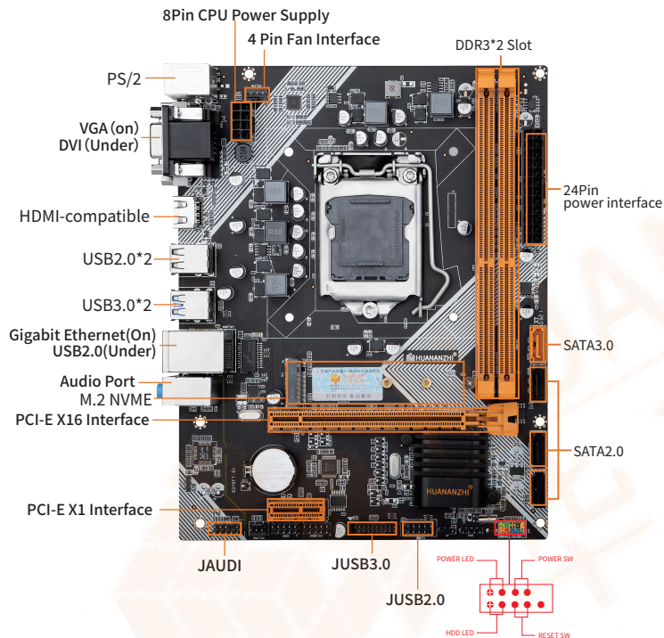
1-1 B75 M.2 Motherboard Illustration
